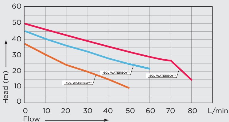
FLOW PERFORMANCE CURVE
