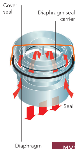
Valve Open (Negative pressure in pipework)
