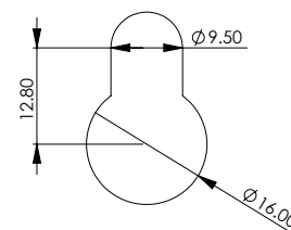
DETAIL A1 ENLARGED MOUNTING HOLE
